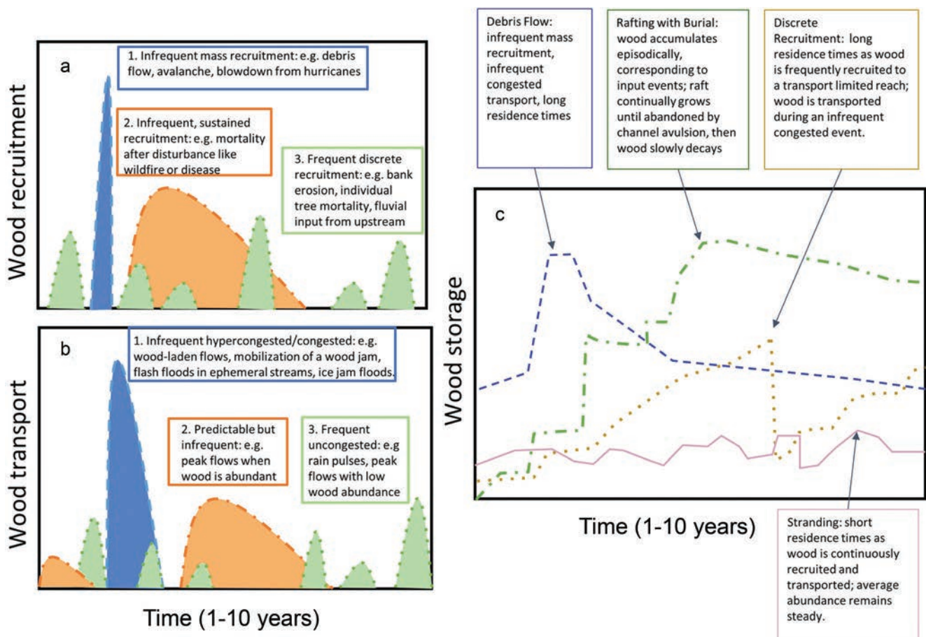
Figure 2. Hypothetical examples of wood recruitment (a), transport (b), and storage (c) regimes through time. Regimes are illustrative: Substantial variability may exist that is not represented in the present article. Wood storage reflects combined interactions between different recruitment and transport regimes. We present expected patterns of storage regimes through time associated with four of the example process domains in figure 3.
