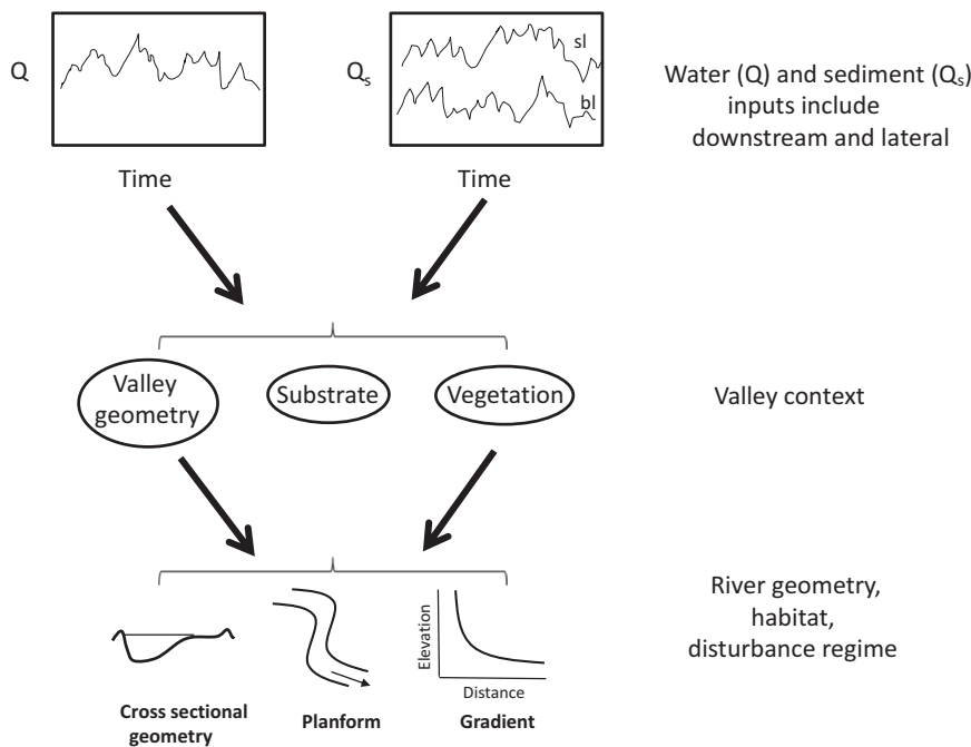
Figure 4. Interactions between water ( Q ) and sediment ( Q_s ), including suspended load ( sl ) and bed-material load ( bl ), discharges in the context of a specific valley configuration and erosional resistance created by substrate and vegetation to influence river geometry. Human alterations at the upper level ( Q , Q_s ) and intermediate level (substrate, vegetation) strongly influence river geometry (the bottom level). River management can manipulate water and sediment discharge and valley context to influence river geometry. Adapted from Thorne (1997).
